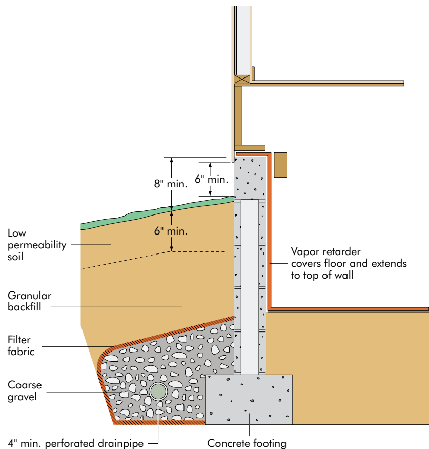
FIGURE 3 CONCRETE MASONRY CRAWL SPACE FOUNDATION
