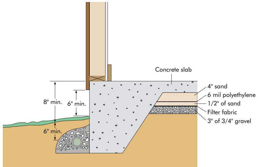
FIGURE 2 SLAB-ON-GRADE FOUNDATION
