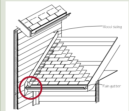
Kick-out flashing (seen in the red circle) diverts water away from the wall and into the gutter.
